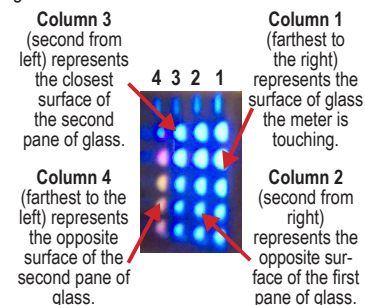
Figure 3: Reflection shown from 2 panes of glass
